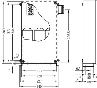
Dimensional drawing LKN Case type 2 (12.5 to 15 kvar)
