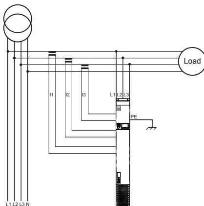
Connection diagram (example)
